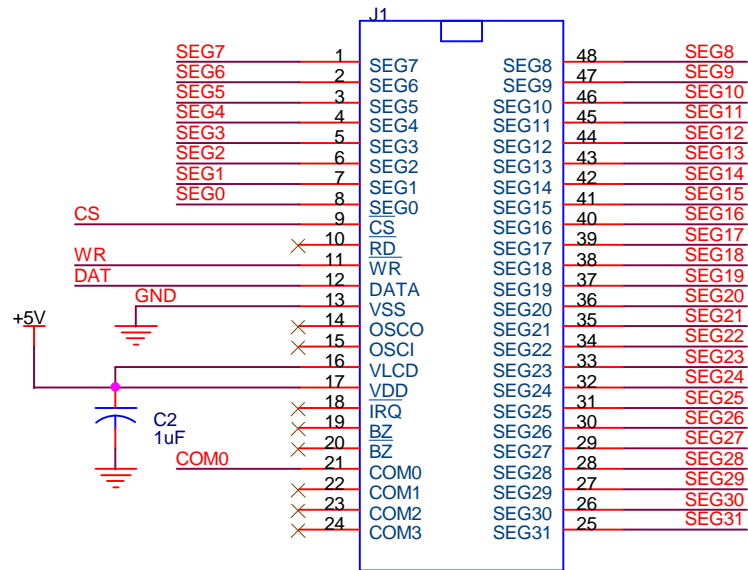
HT1621B 48 SSOP-A
