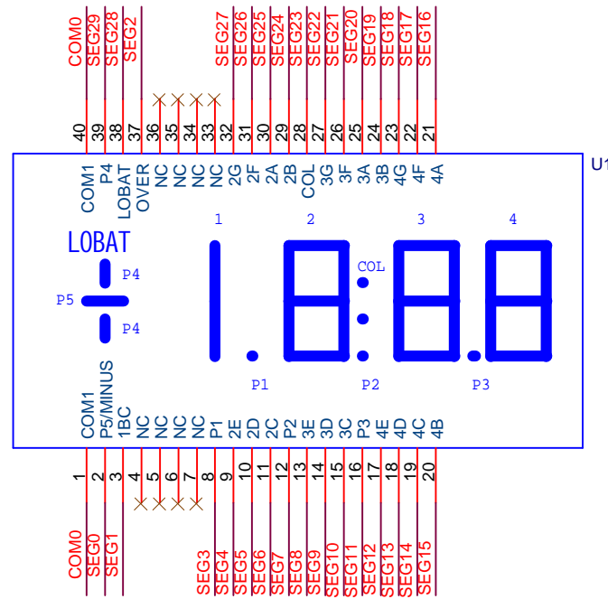
3 1/2 DIGIT LCD (+5V VERSION)
