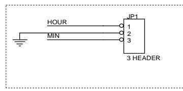
Optional remote set time switch on-off-on
